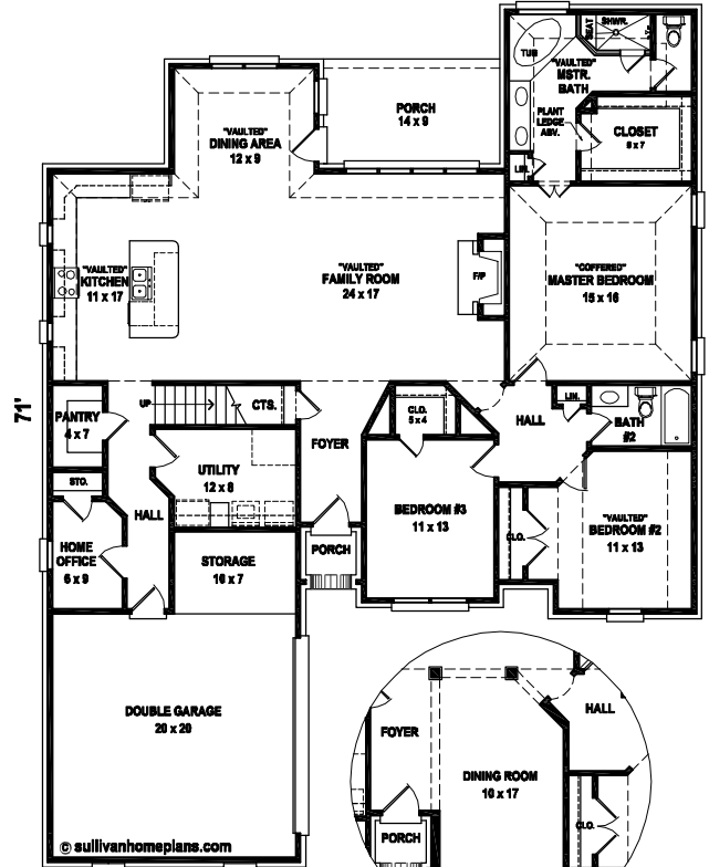
FIRST LEVEL FLOOR PLAN
