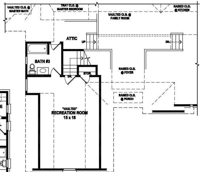
SECOND LEVEL FLOOR PLAN
