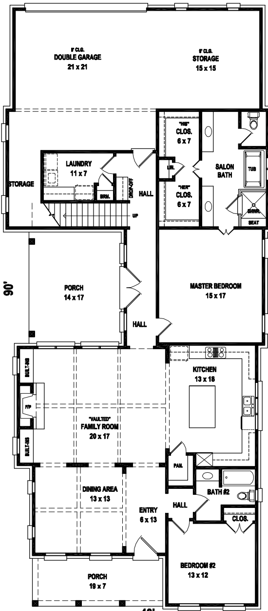
FIRST LEVEL FLOOR PLAN
